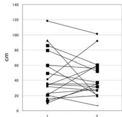
Figure6 The comparison of before and after head change position of the walk test (n=18) 1:Horizontal head position 2:30 degree inclined forward head position
